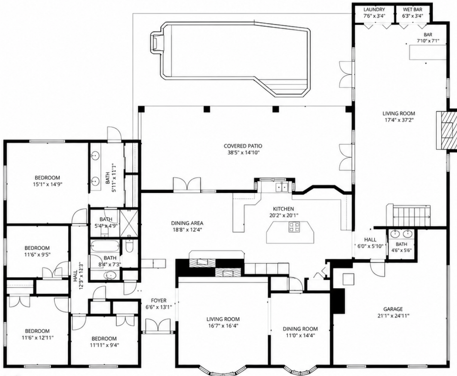
1st floor
