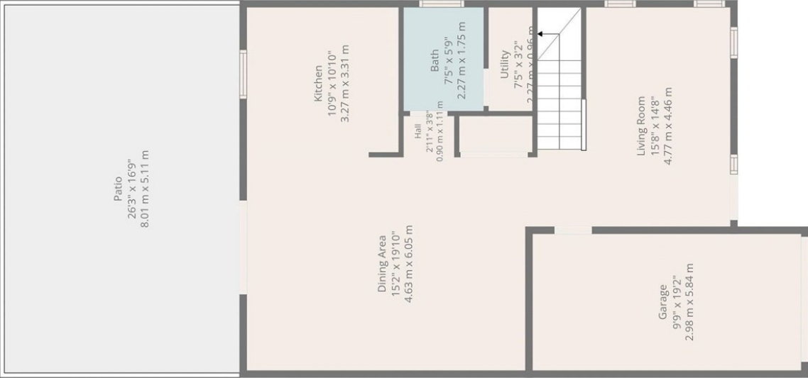
1st Floor
