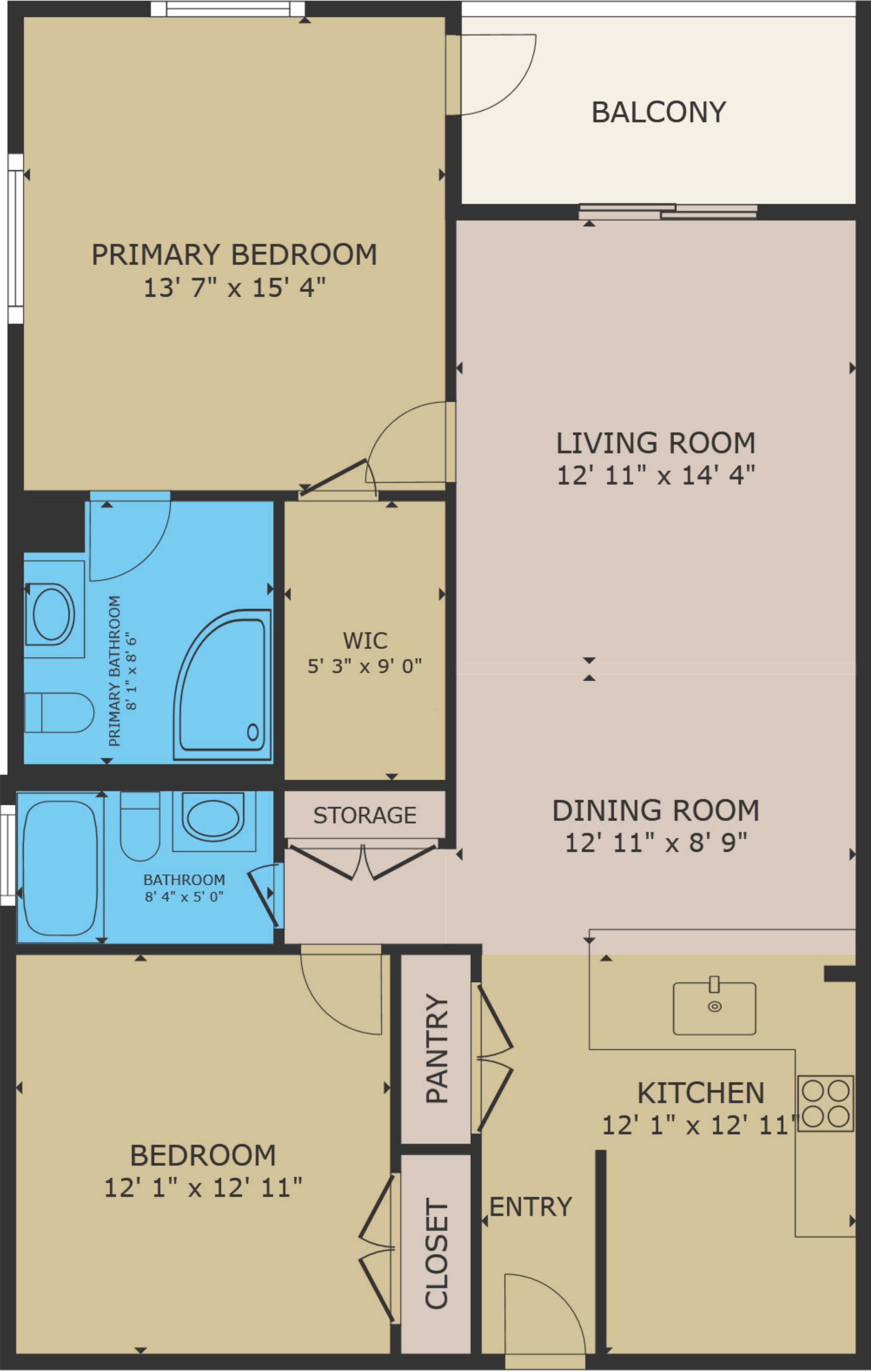
FLOOR PLAN
