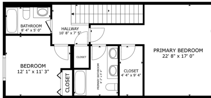
FLOOR 2
